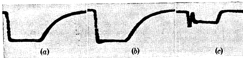
FIG. 8-32.—Voltage and current pulses taken with \frac{1}{2} - \mu sec pulser having a rapid voltage rise. (a) Voltage below oscillating region; (b) voltage pulse in oscillating region; (c) current pulse in oscillating region.
